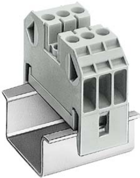
THROUGH-TYPE TERMINAL THERMOPL. SCREW TERMINAL ON BOTH ENDS TERMINAL BLOCK 3-POLE, BEIGE 18MM, SZ 2.5
