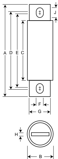
Fig. 1: 35-800 Amp Range
