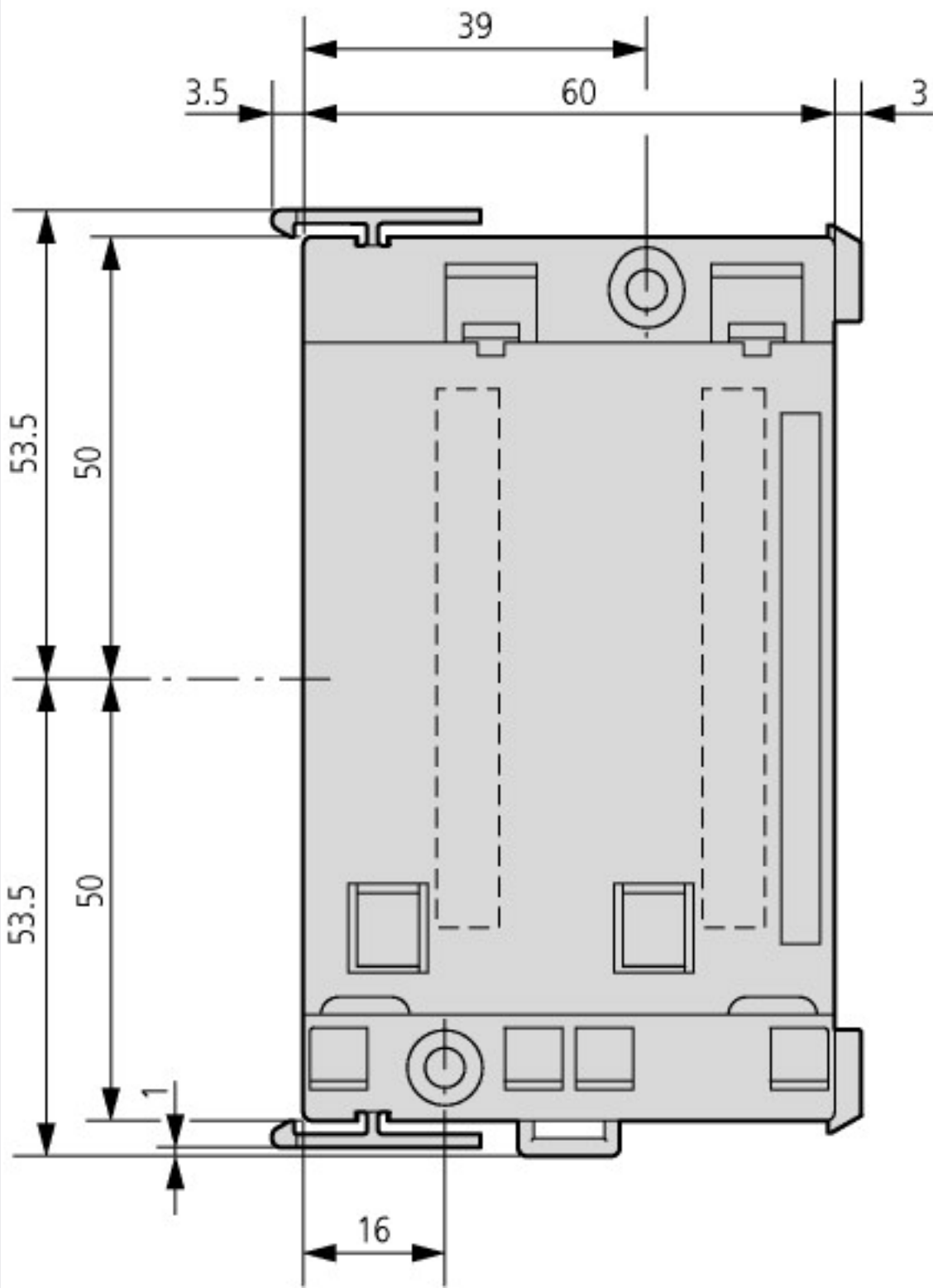
Racks
